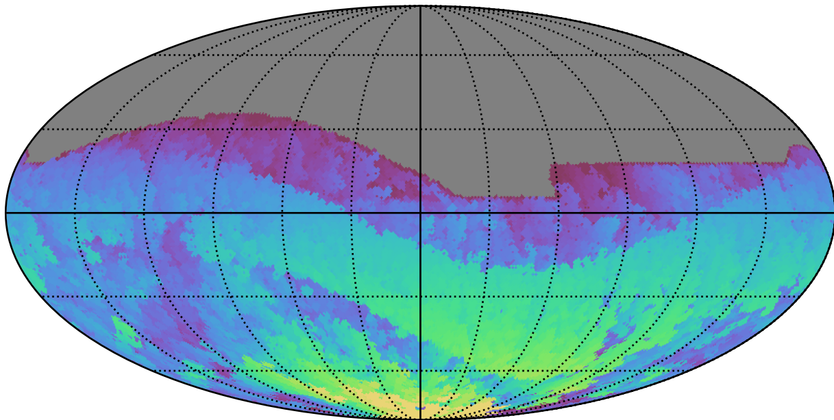
noroll_mjdp120_v3.4_10yrs All sky z band: Max HA
