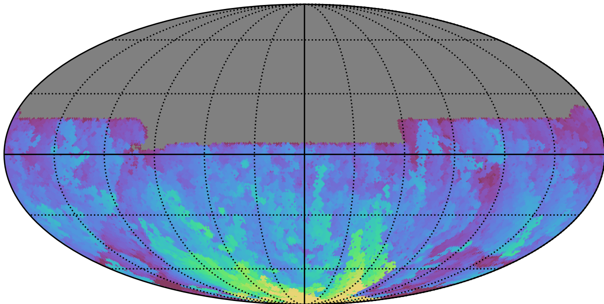
noroll_mjdp120_v3.4_10yrs All sky u band: Max HA
