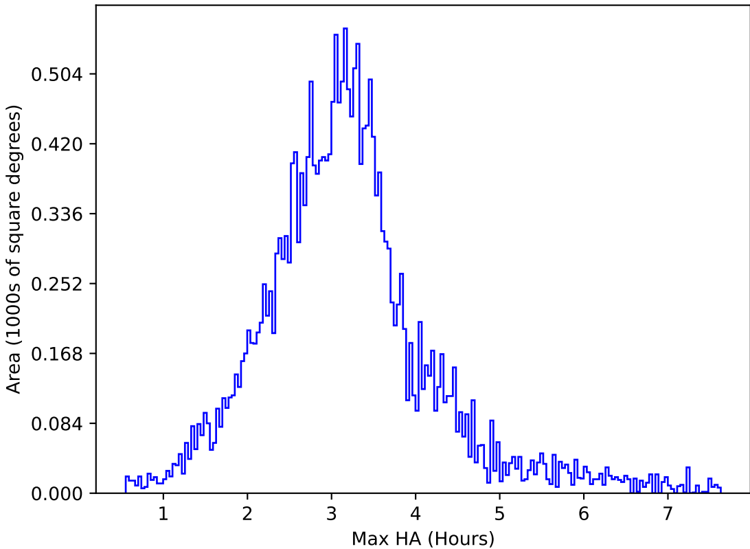
noroll_mjdp120_v3.4_10yrs All sky u band: Max HA
