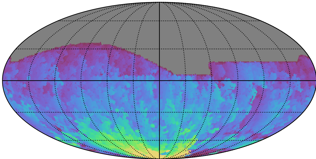
noroll_mjdp120_v3.4_10yrs All sky r band: Max HA
