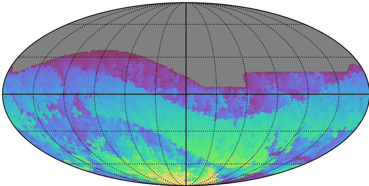
noroll_mjdp120_v3.4_10yrs All sky i band: Max HA
