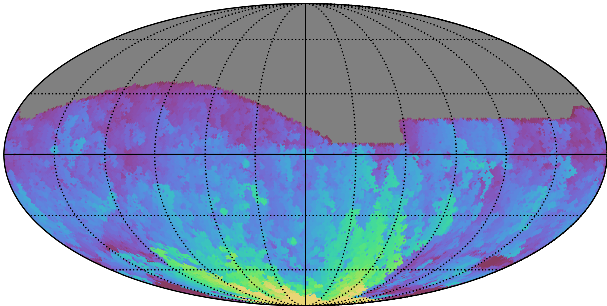
noroll_mjdp120_v3.4_10yrs All sky g band: Max HA
