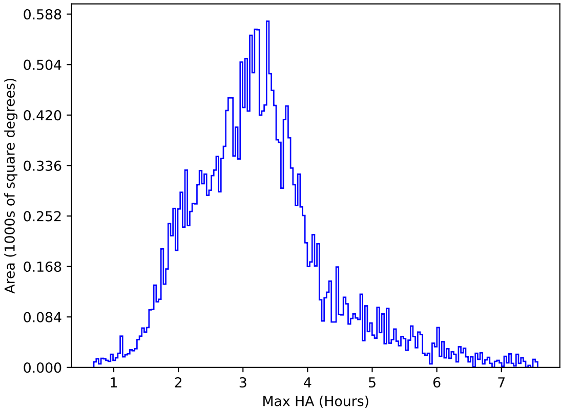
noroll_mjdp120_v3.4_10yrs All sky g band: Max HA
