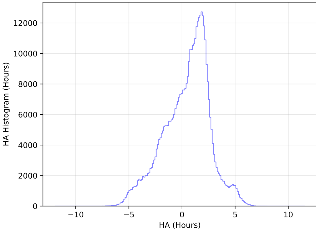
noroll_mjdp120_v3.4_10yrs WFD z band: HA Histogram
