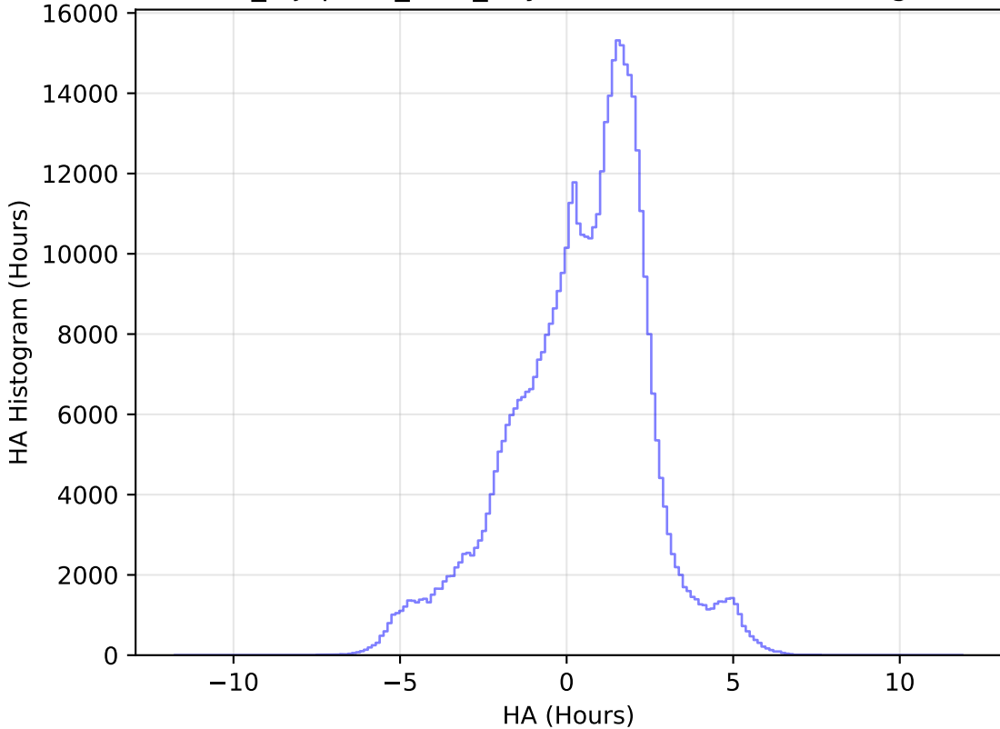
noroll_mjdp120_v3.4_10yrs WFD i band: HA Histogram
