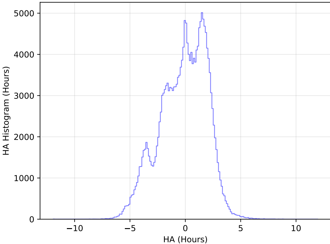
noroll_mjdp120_v3.4_10yrs WFD g band: HA Histogram
