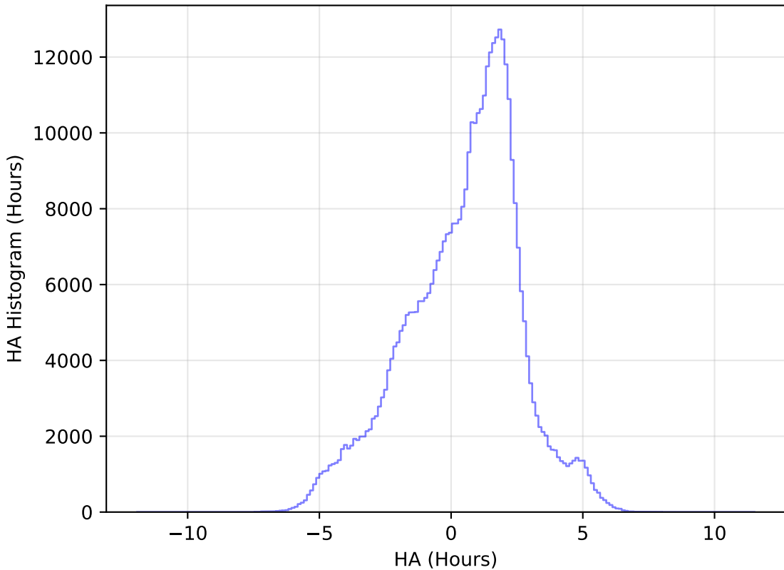
noroll_mjdp120_v3.4_10yrs All sky z band: HA Histogram
