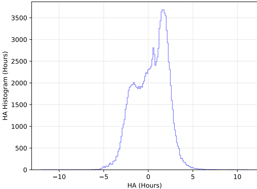
noroll_mjdp120_v3.4_10yrs All sky u band: HA Histogram
