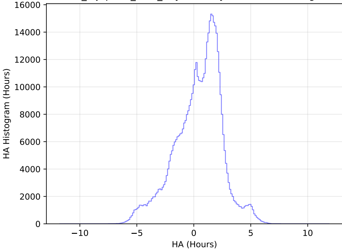
noroll_mjdp120_v3.4_10yrs All sky i band: HA Histogram
