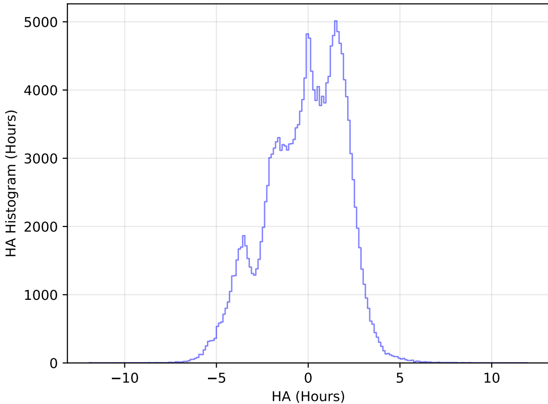
noroll_mjdp120_v3.4_10yrs All sky g band: HA Histogram
