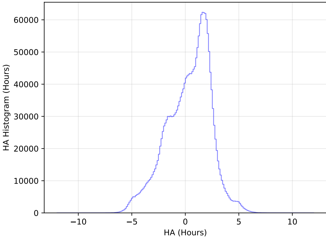
noroll_mjdp120_v3.4_10yrs All sky all bands: HA Histogram
