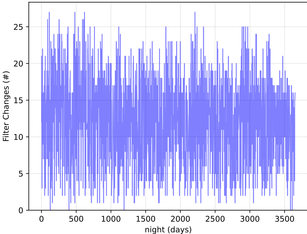
noroll_mjdp120_v3.4_10yrs Per Night: Filter Changes
