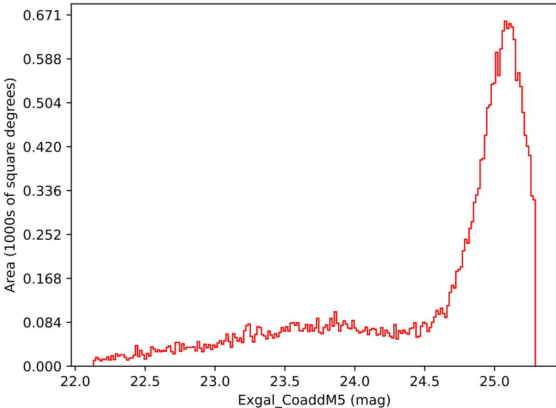
noroll_mjdp120_v3.4_10yrs Yr 3-4 i band: Exgal_CoaddM5
