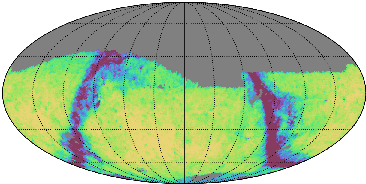
noroll_mjdp120_v3.4_10yrs Yr 3-4 g band: Exgal_CoaddM5
