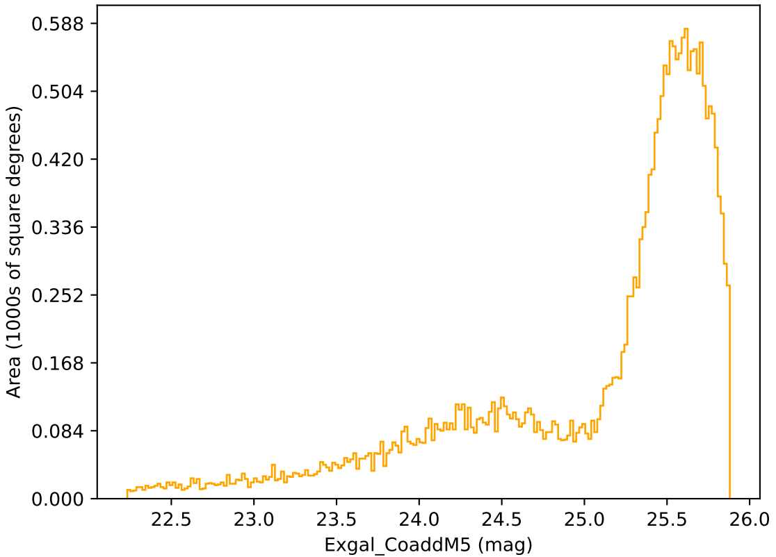
noroll_mjdp120_v3.4_10yrs Yr 1 r band: Exgal_CoaddM5
