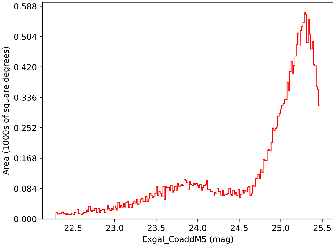
noroll_mjdp120_v3.4_10yrs Yr 1 i band: Exgal_CoaddM5
