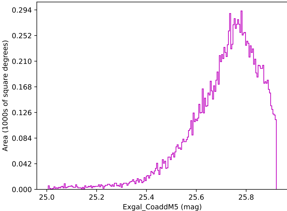
noroll_mjdp120_v3.4_10yrs WFD z band: Exgal_CoaddM5
