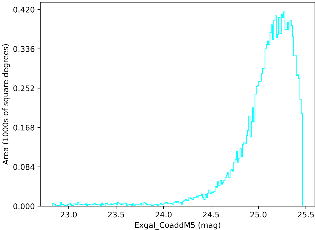
noroll_mjdp120_v3.4_10yrs WFD u band: Exgal_CoaddM5
