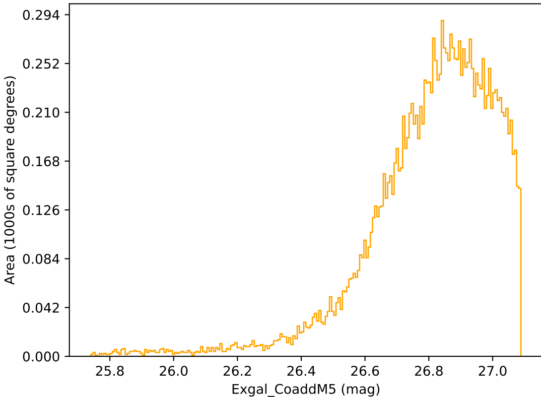
noroll_mjdp120_v3.4_10yrs WFD r band: Exgal_CoaddM5
