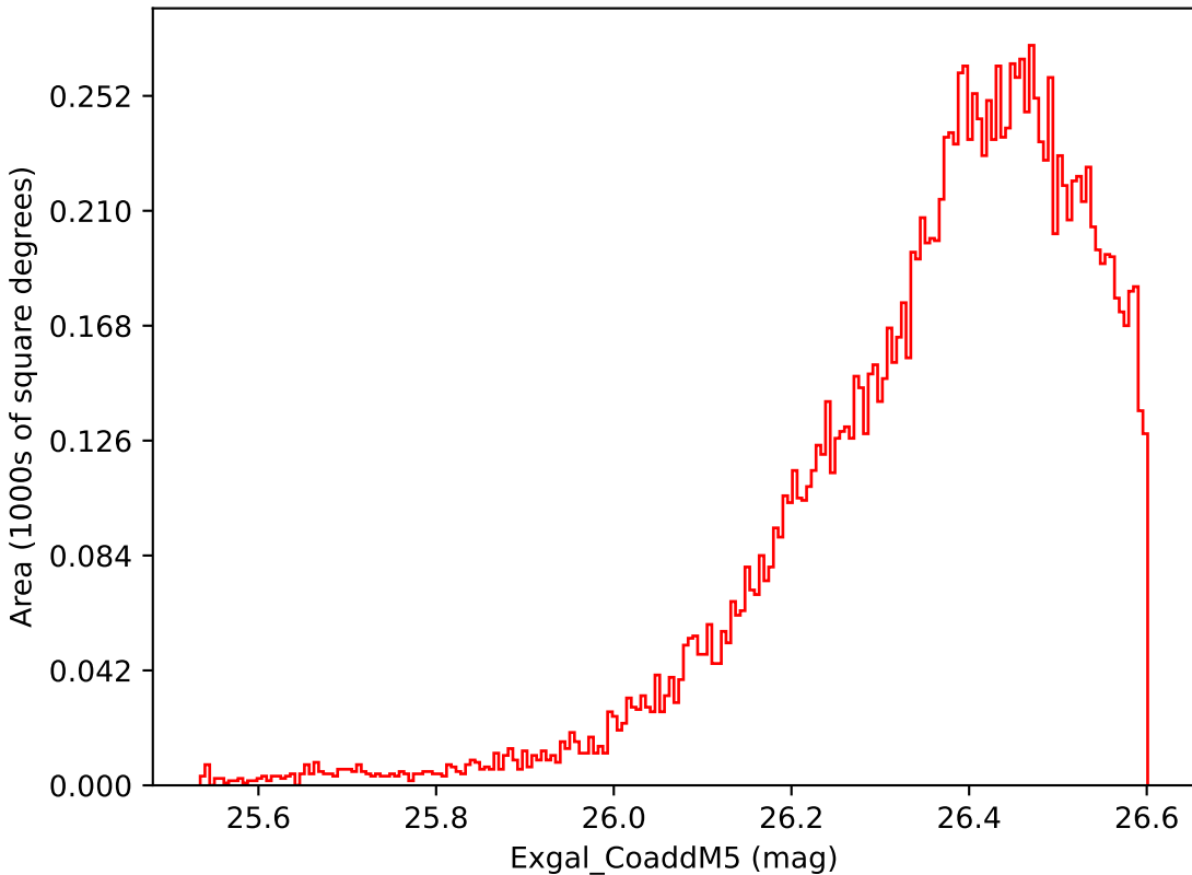
noroll_mjdp120_v3.4_10yrs WFD i band: Exgal_CoaddM5
