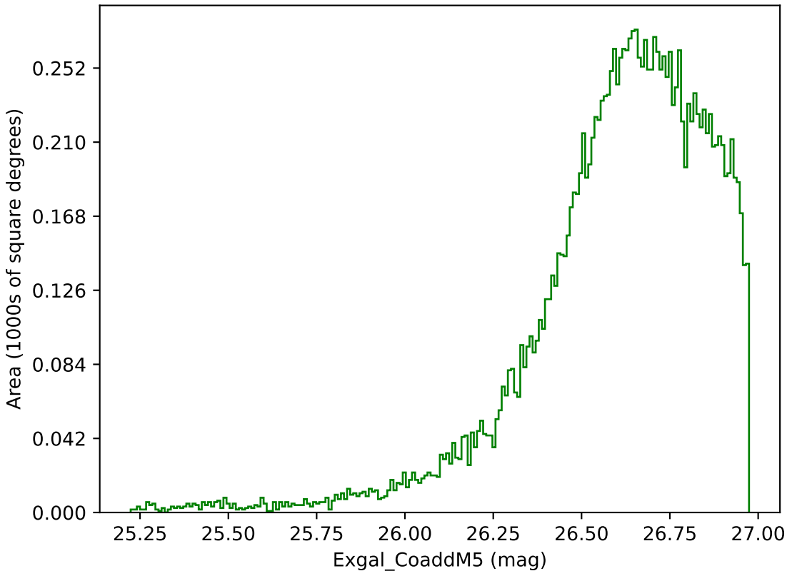
noroll_mjdp120_v3.4_10yrs WFD g band: Exgal_CoaddM5
