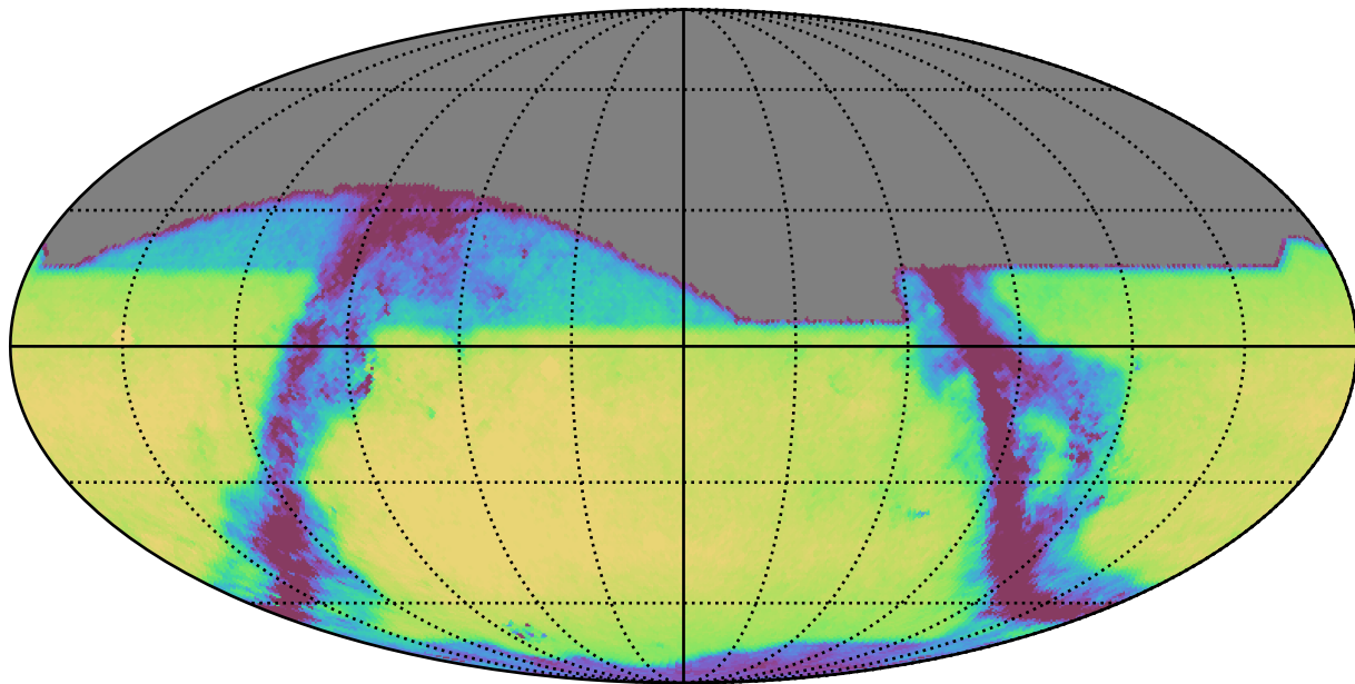
noroll_mjdp120_v3.4_10yrs All sky z band: Exgal_CoaddM5
