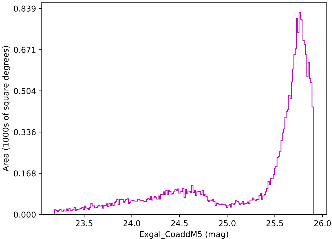
noroll_mjdp120_v3.4_10yrs All sky z band: Exgal_CoaddM5
