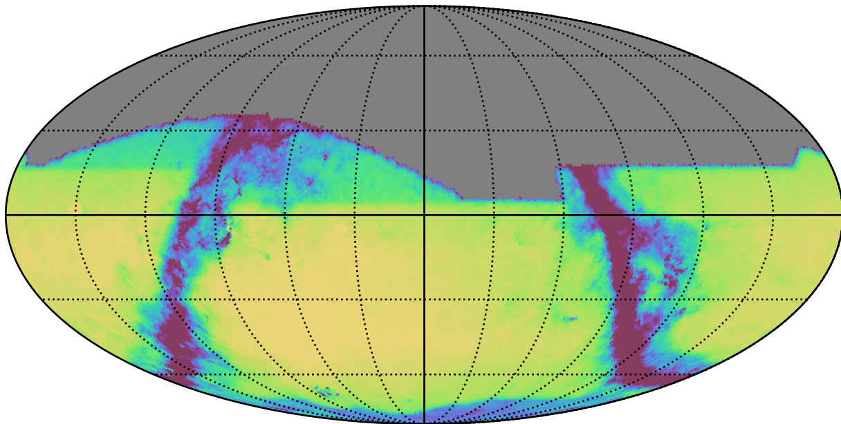
noroll_mjdp120_v3.4_10yrs All sky r band: Exgal_CoaddM5
