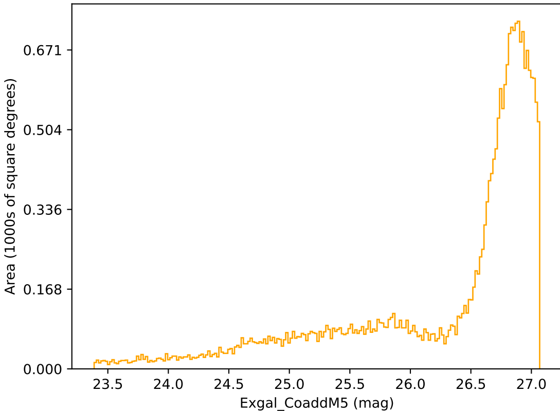
noroll_mjdp120_v3.4_10yrs All sky r band: Exgal_CoaddM5
