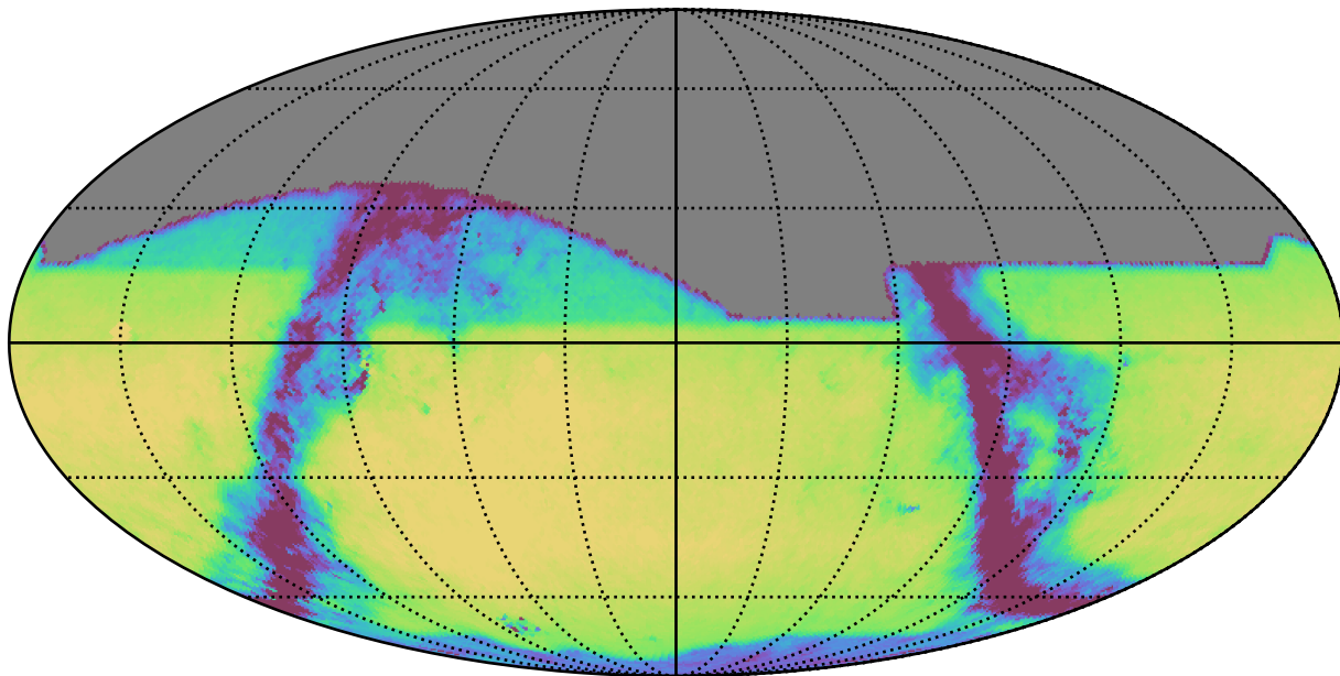
noroll_mjdp120_v3.4_10yrs All sky i band: Exgal_CoaddM5
