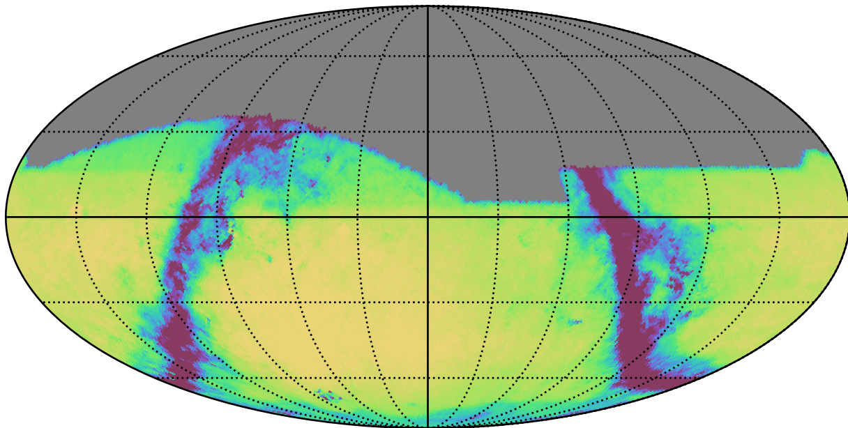
noroll_mjdp120_v3.4_10yrs All sky g band: Exgal_CoaddM5
