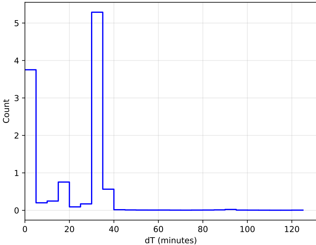
1e6 noroll_mjdp120_v3.4_10yrs WFD: DeltaT Histogram
