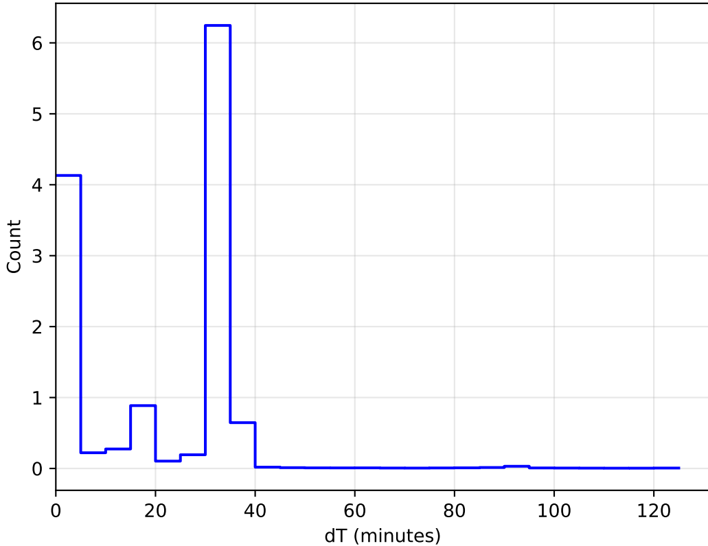
noroll_mjdp120_v3.4_10yrs All sky: DeltaT Histogram
