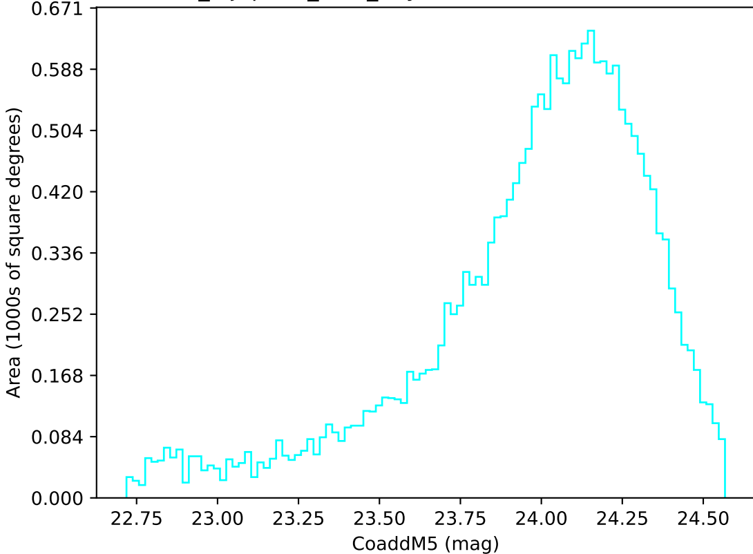
noroll_mjdp120_v3.4_10yrs Yr 3-4 u band: CoaddM5
