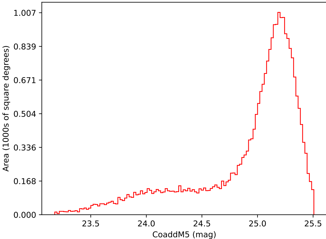
noroll_mjdp120_v3.4_10yrs Yr 3-4 i band: CoaddM5
