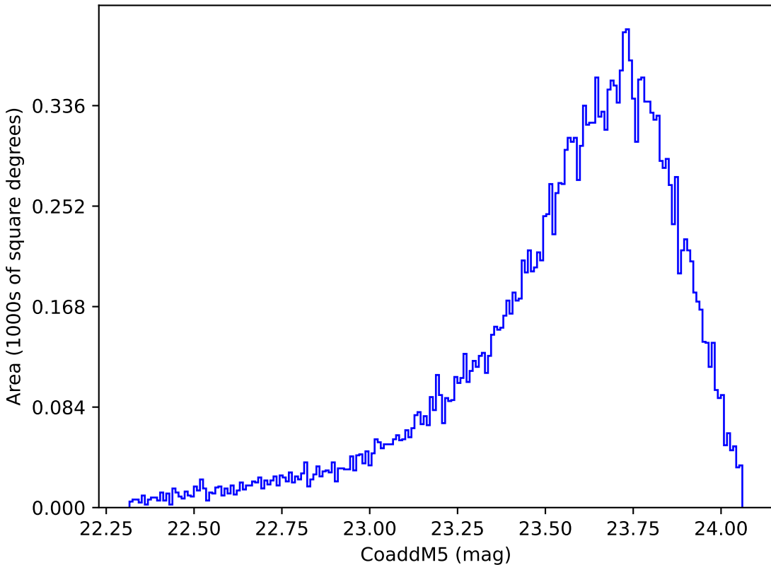
noroll_mjdp120_v3.4_10yrs Yr 1 y band: CoaddM5
