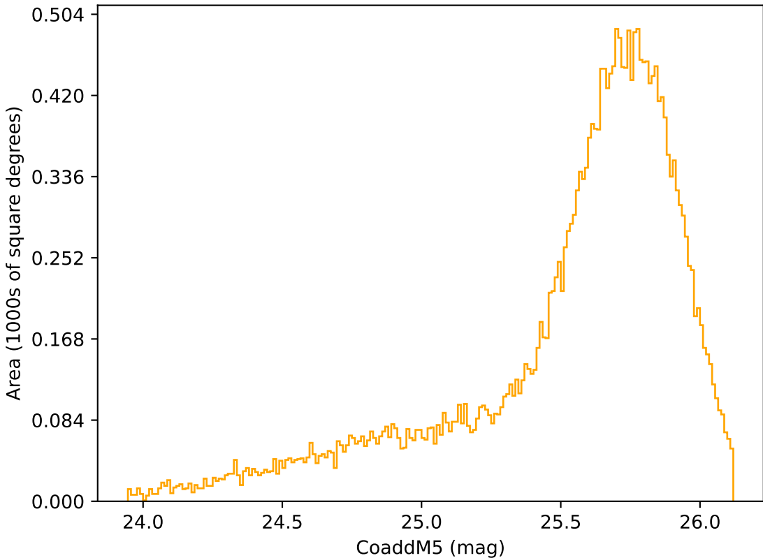
noroll_mjdp120_v3.4_10yrs Yr 1 r band: CoaddM5
