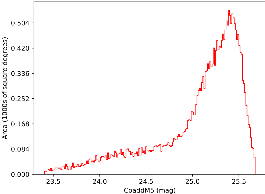
noroll_mjdp120_v3.4_10yrs Yr 1 i band: CoaddM5
