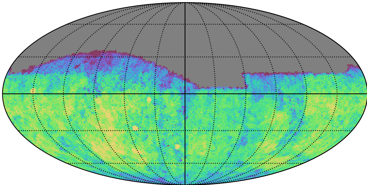
noroll_mjdp120_v3.4_10yrs Yr 1 g band: CoaddM5
