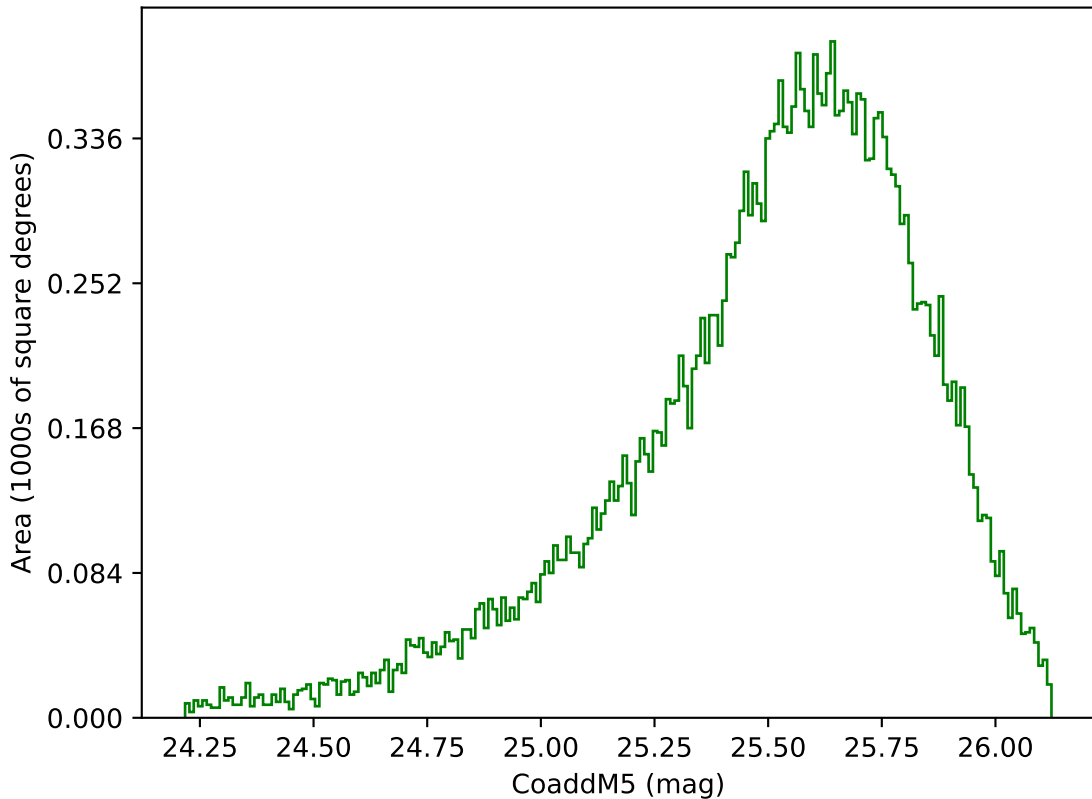
noroll_mjdp120_v3.4_10yrs Yr 1 g band: CoaddM5
