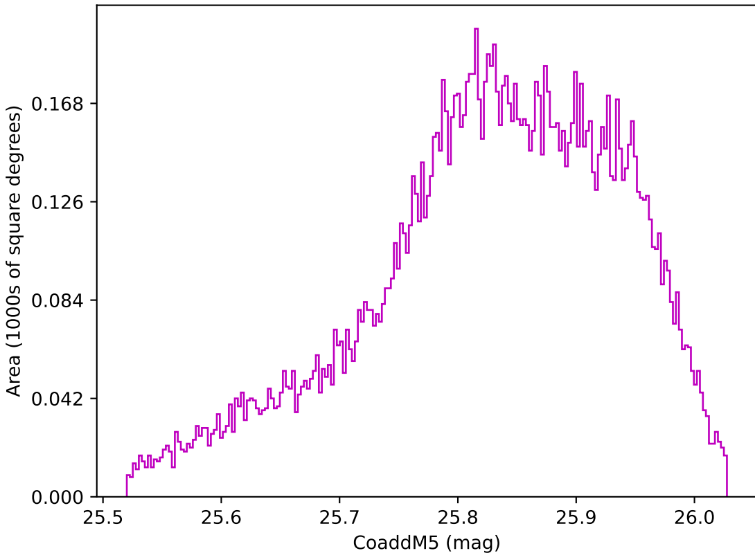
noroll_mjdp120_v3.4_10yrs WFD z band: CoaddM5
