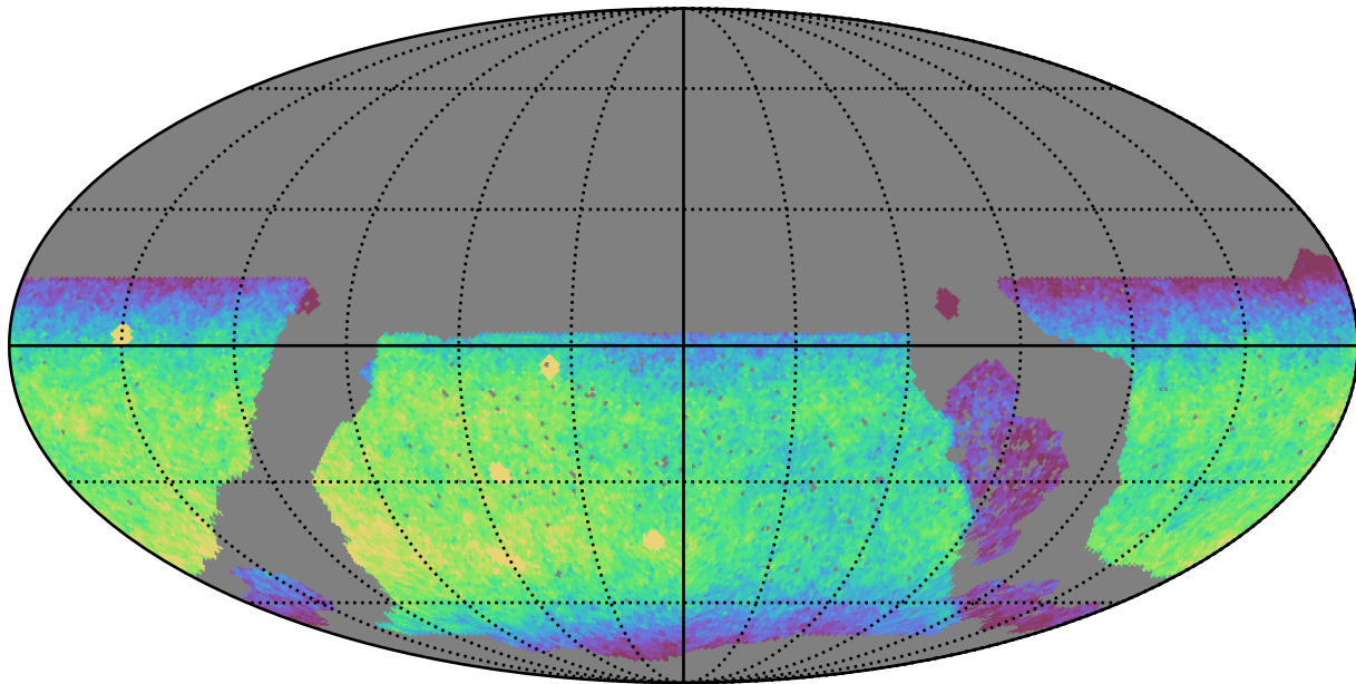
noroll_mjdp120_v3.4_10yrs WFD y band: CoaddM5
