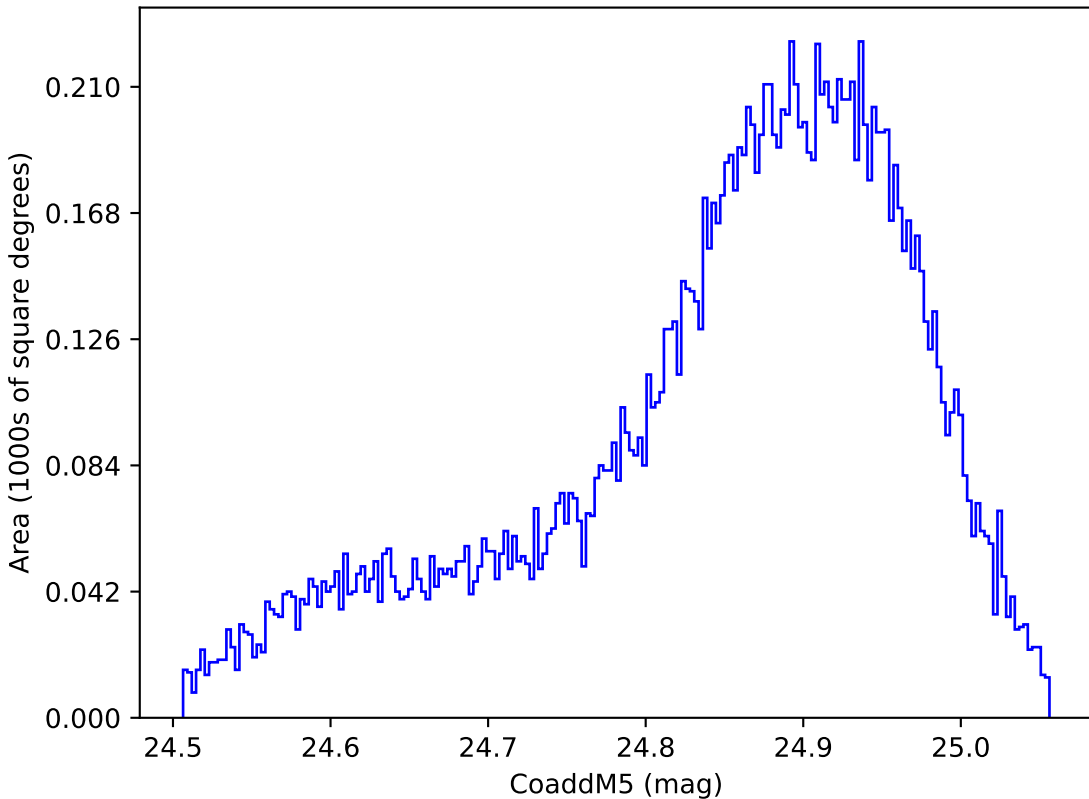
noroll_mjdp120_v3.4_10yrs WFD y band: CoaddM5
