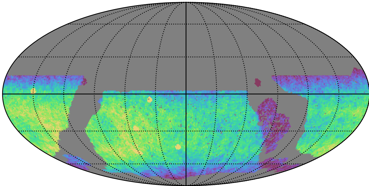
noroll_mjdp120_v3.4_10yrs WFD u band: CoaddM5
