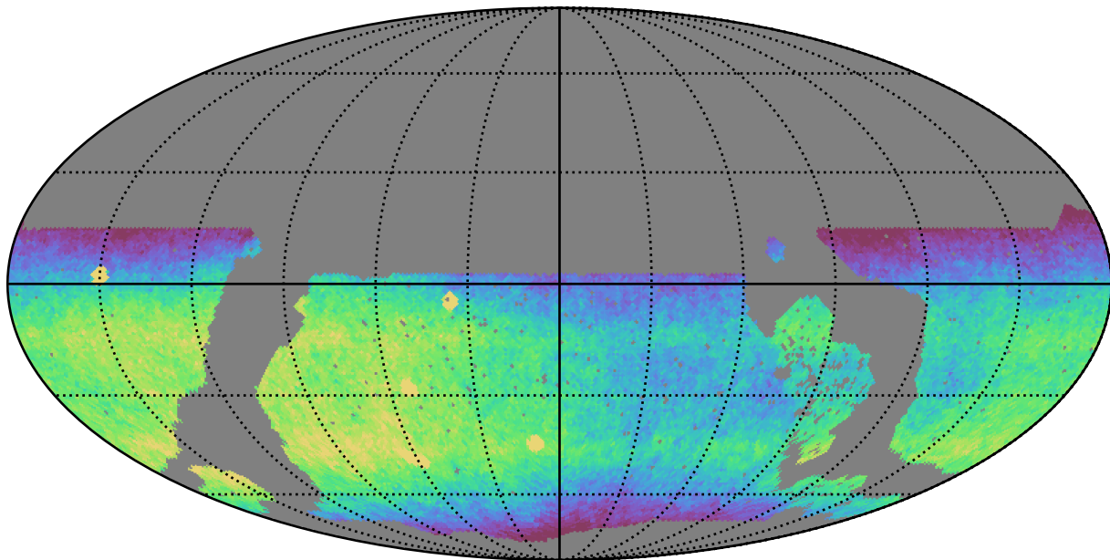
noroll_mjdp120_v3.4_10yrs WFD r band: CoaddM5
