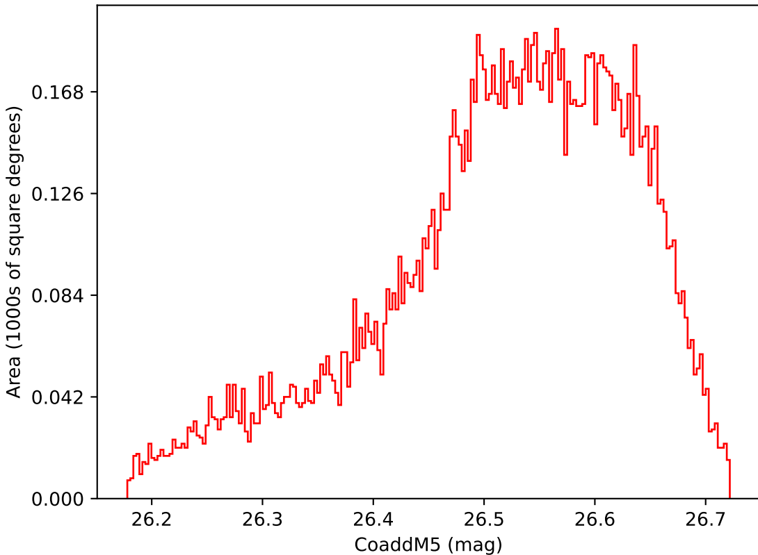
noroll_mjdp120_v3.4_10yrs WFD i band: CoaddM5
