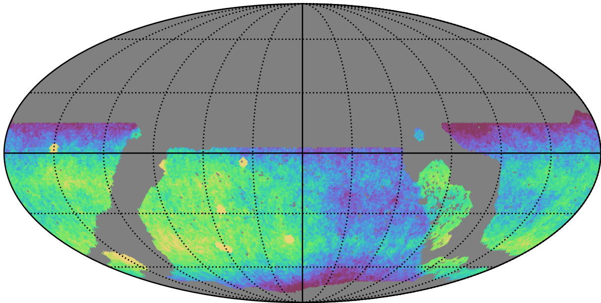
noroll_mjdp120_v3.4_10yrs WFD g band: CoaddM5
