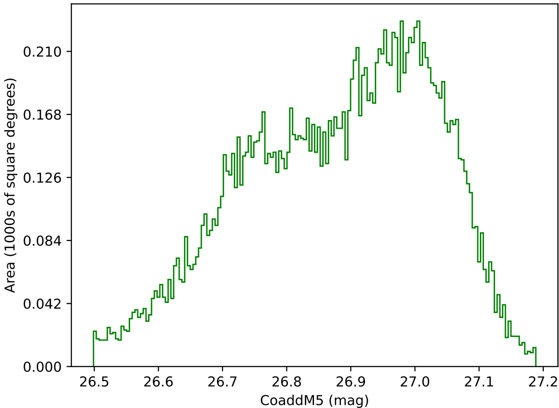
noroll_mjdp120_v3.4_10yrs WFD g band: CoaddM5
