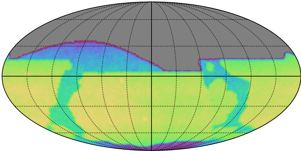
noroll_mjdp120_v3.4_10yrs All sky z band: CoaddM5
