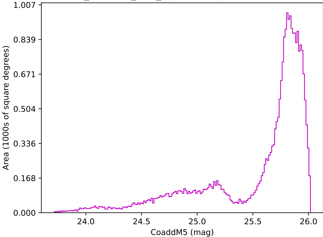
noroll_mjdp120_v3.4_10yrs All sky z band: CoaddM5
